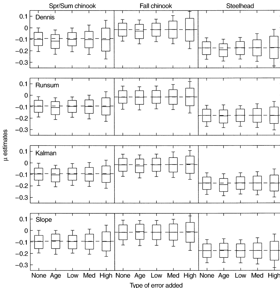
FIG. 2. Performance of the \mu estimates from the Dennis, runsum, Kalman, and slope methods. One thousand 20-year spawner time series were generated from the spring/summer chinook, fall chinook, and steelhead stochastic matrix models. The column labels indicate the type of error added: “None” indicates stable starting age structure and no sampling error; “Age” indicates no sampling error but perturbed age structure; “Low,” “Med,” and “High” indicate stable age structure plus lognormal sampling error with \sigma_{se}^2 = 0.1, 0.5, \text{ or } 0.75 , respectively. The box plots summarize the estimates among all 1000 simulations. The line in the box shows the median estimates, and the box encloses the middle 75% of the estimates; the whiskers enclose 95% of the estimates.
